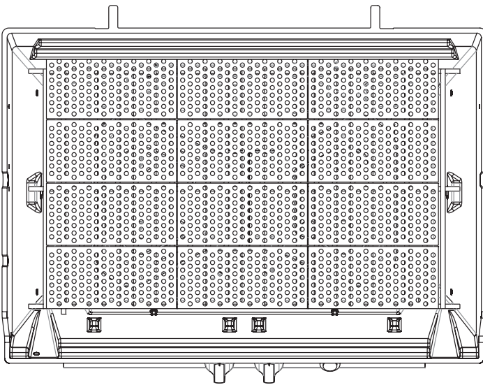
Flare Buster Ceramic Layout for P3 Series Grills
