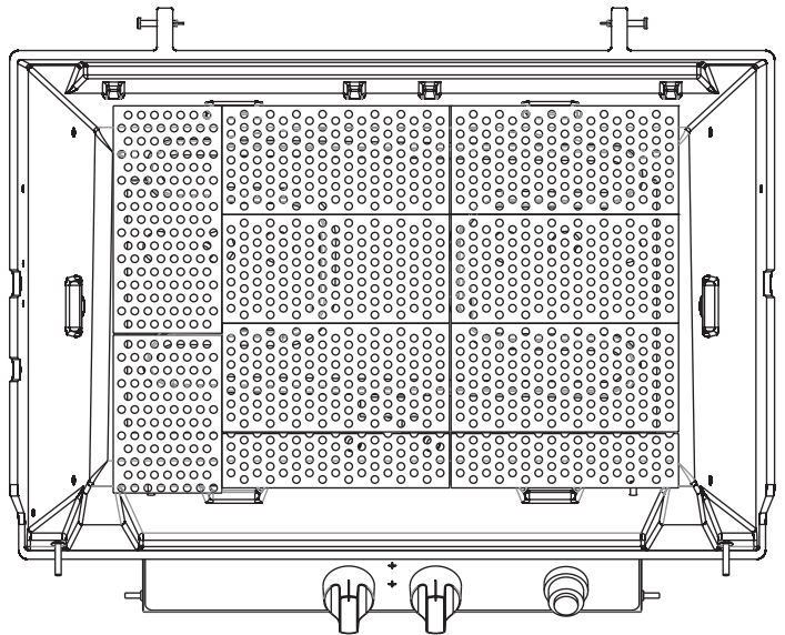
Flare Buster Ceramic Layout for P4 Series Grills
